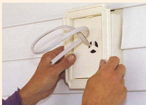
Utility boxes create receiving channels. A snap-on molding holds panel ends around a light box near the front door.
